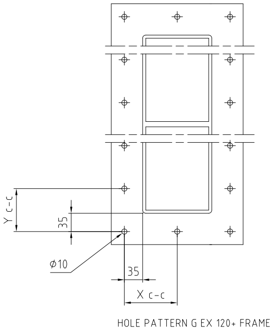
HOLE PATTERN G EX 120+ FRAME
